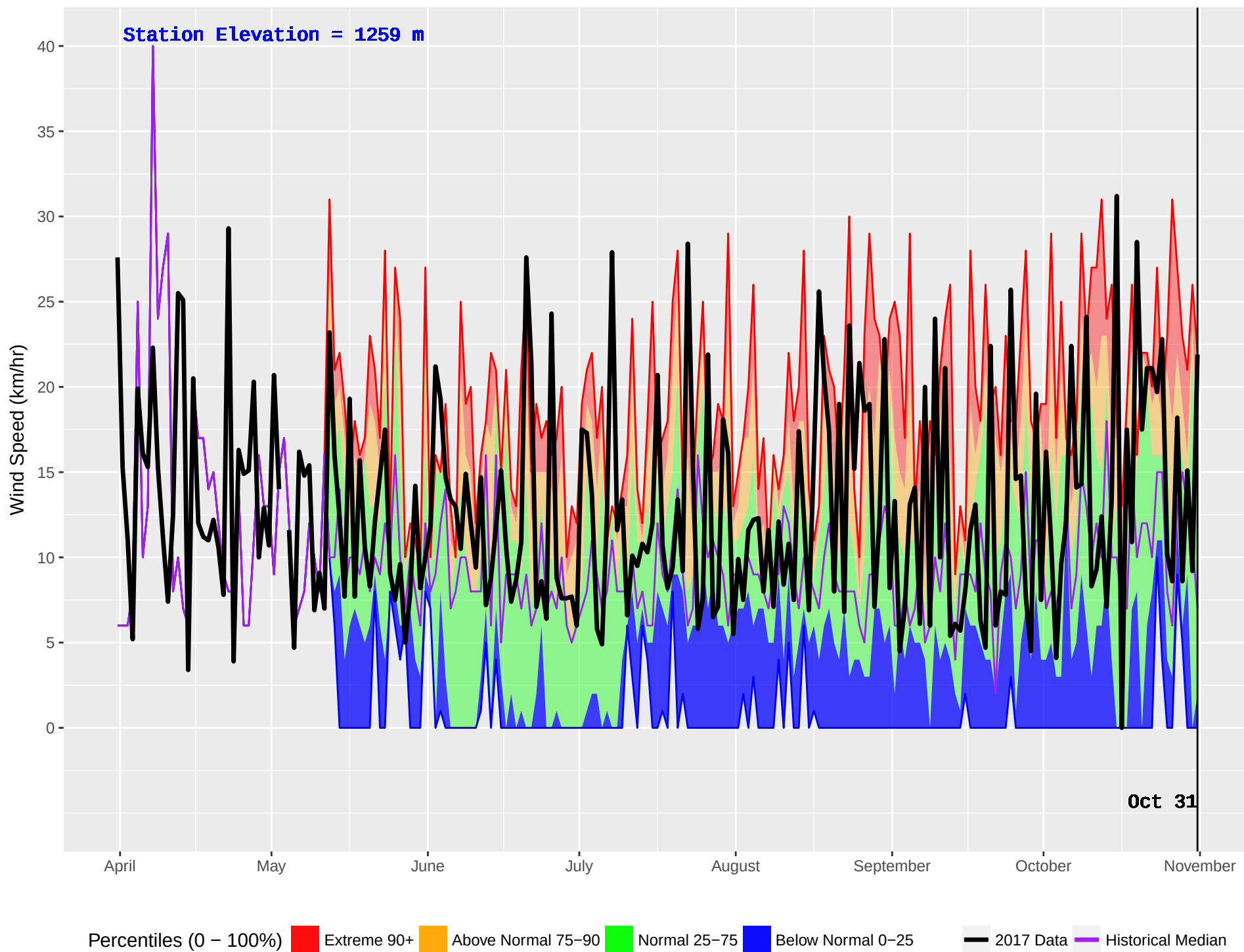
PARROTT (183) : Historical (1995–2016) and Current (2017) Noon Wind Speed
