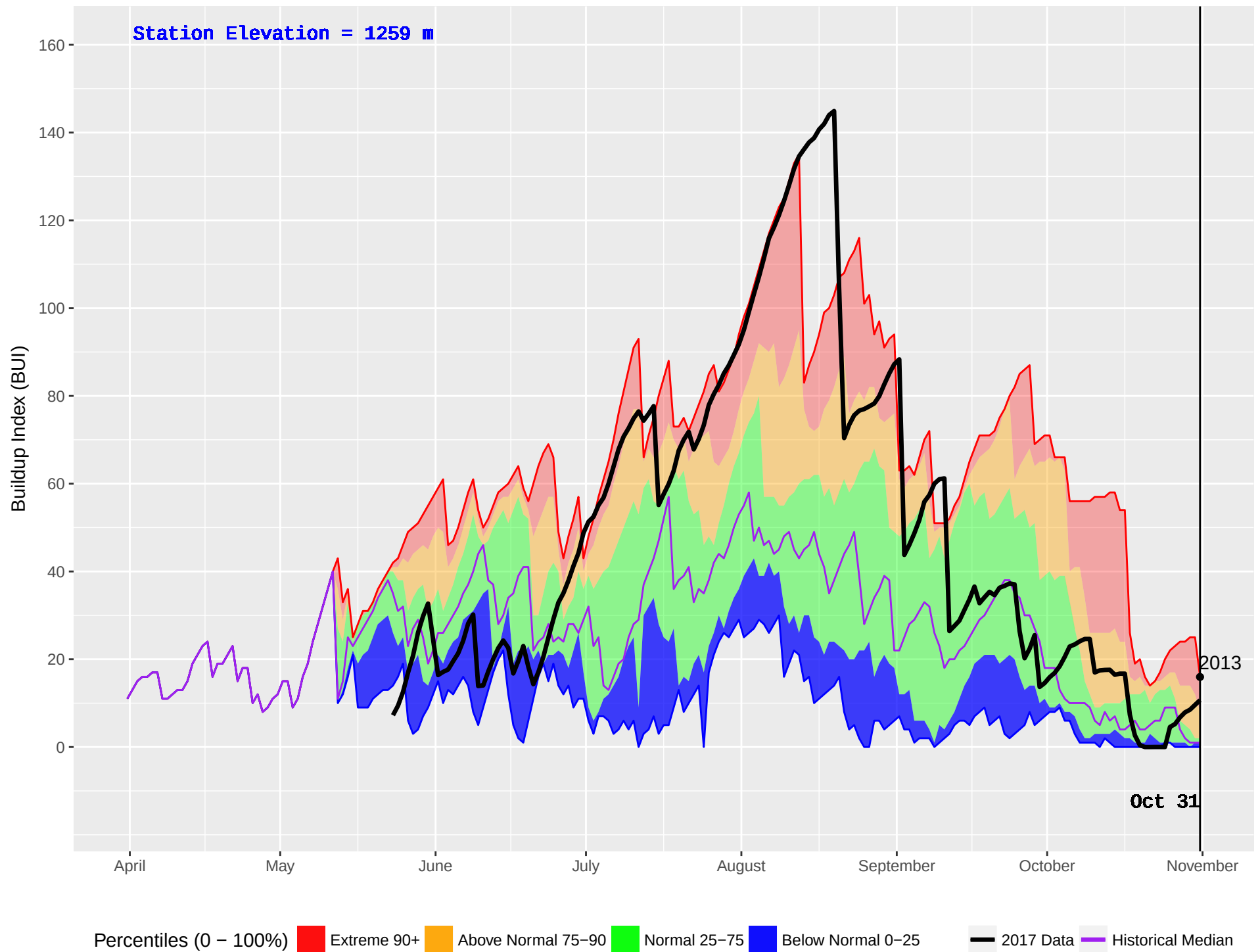
PARROTT (183) : Historical (1995–2016) and Current (2017) Noon Buildup Index (BUI)
