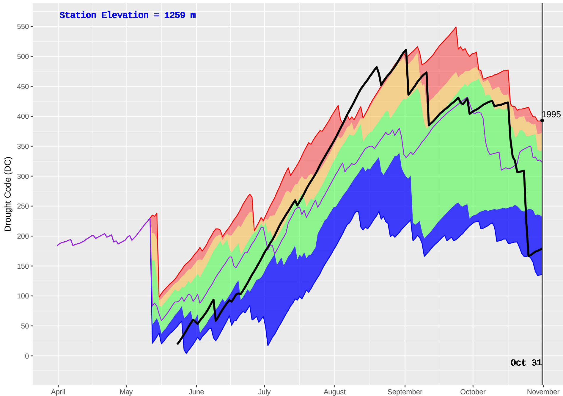
PARROTT (183) : Historical (1995–2016) and Current (2017) Noon Drought Code (DC)
